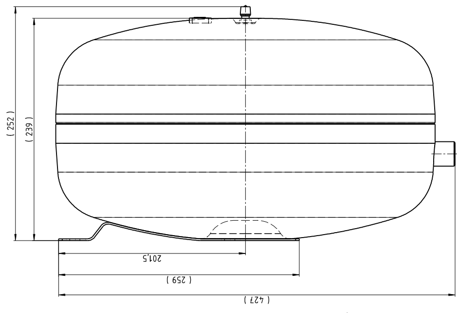
Front view Scale 1:5
