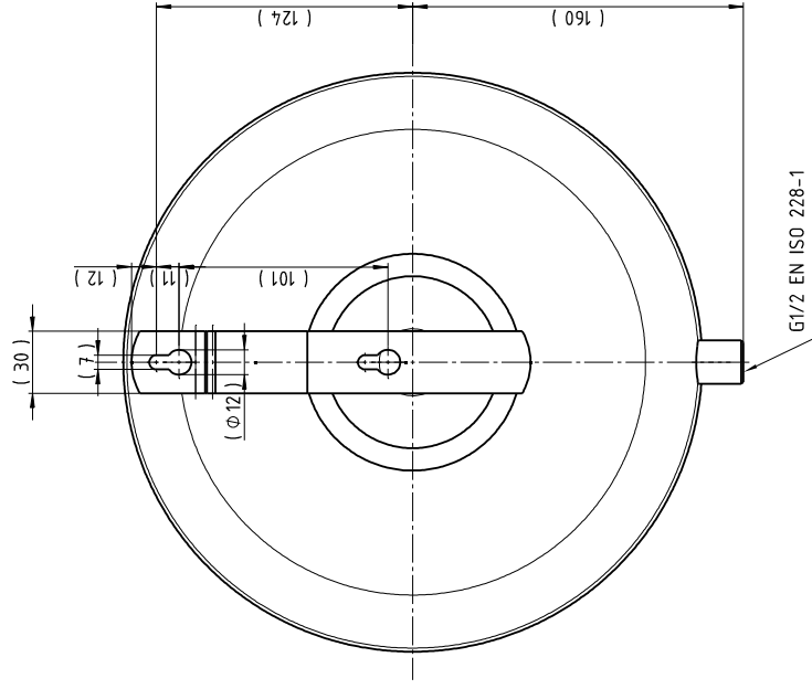
Rear view
