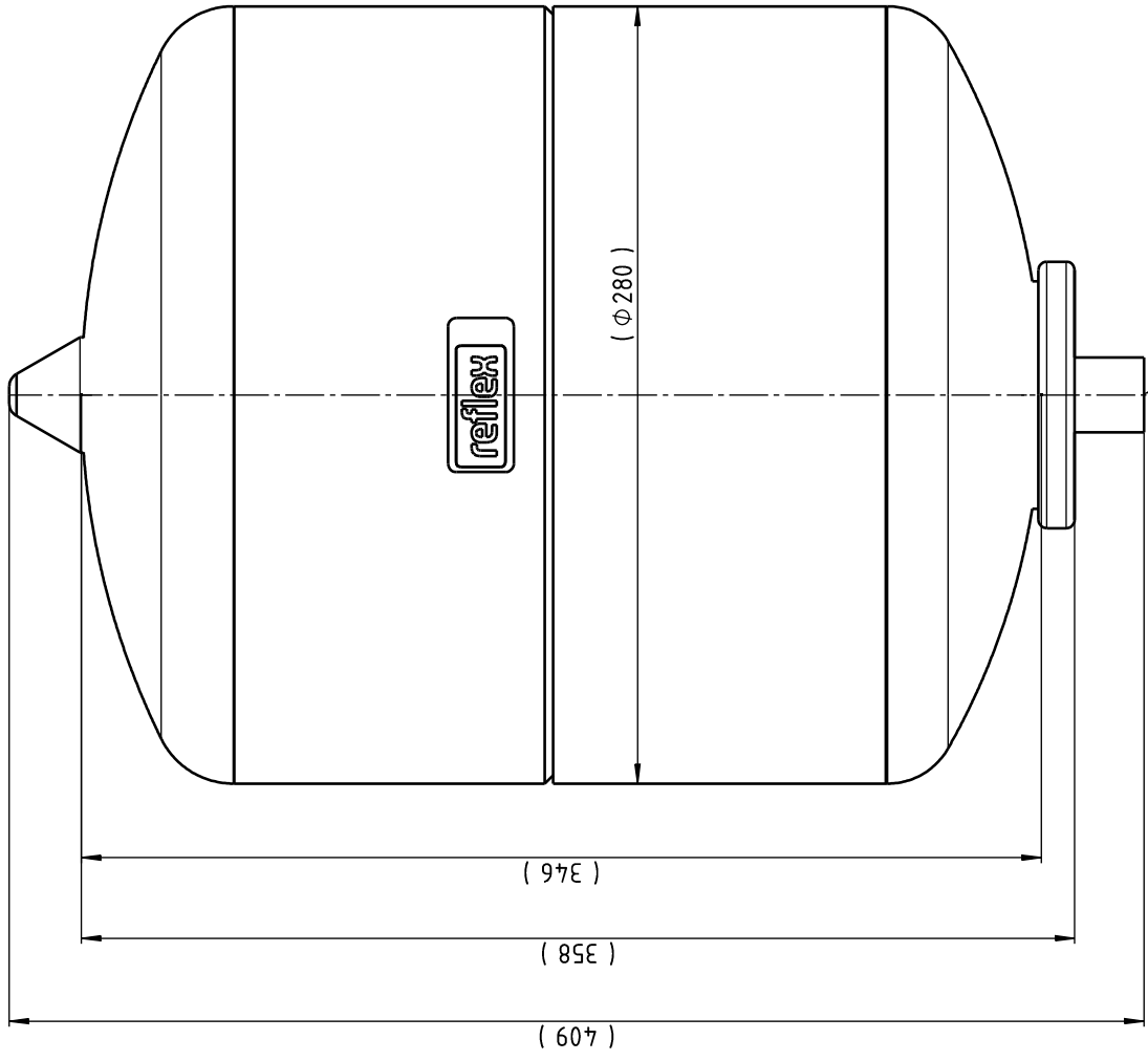
Front view
